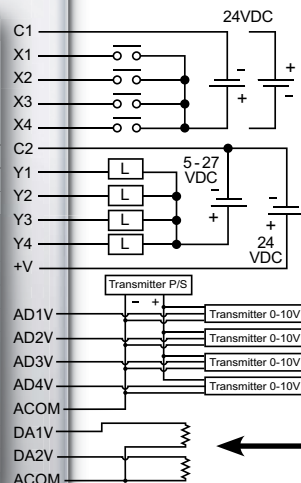
Wiring Diagram
