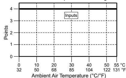
C0-12DD1E-1-D Temperature Derating Chart
