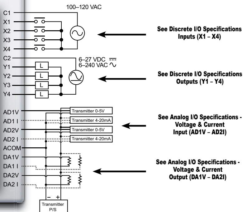
Wiring Diagram
