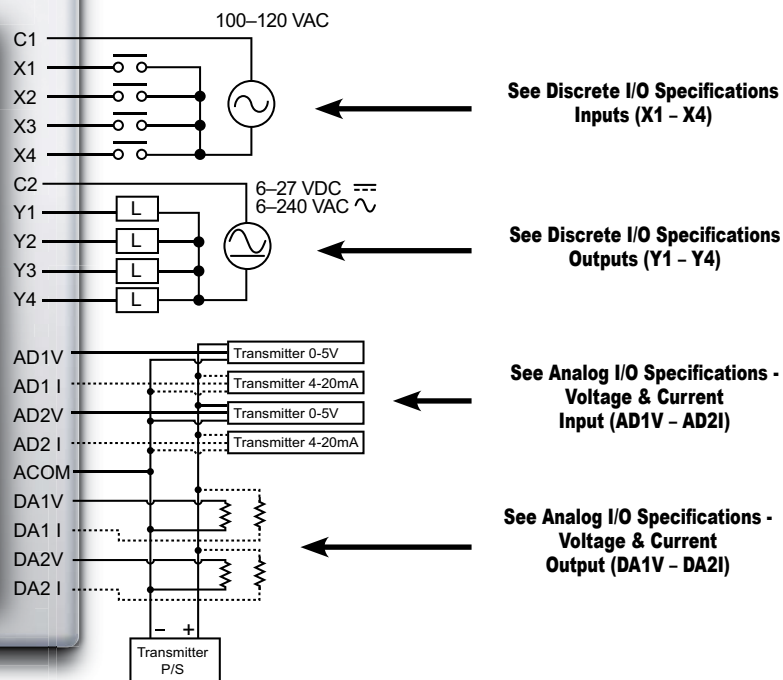
Wiring Diagram
