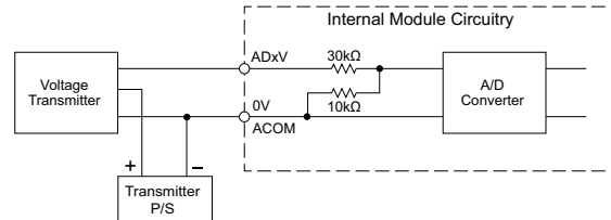
Analog Voltage Input Circuit
