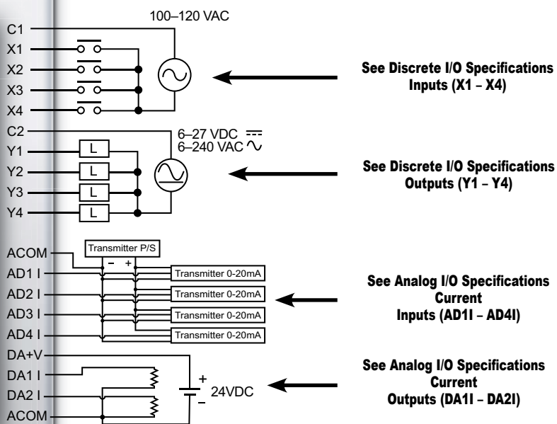
Wiring Diagram
