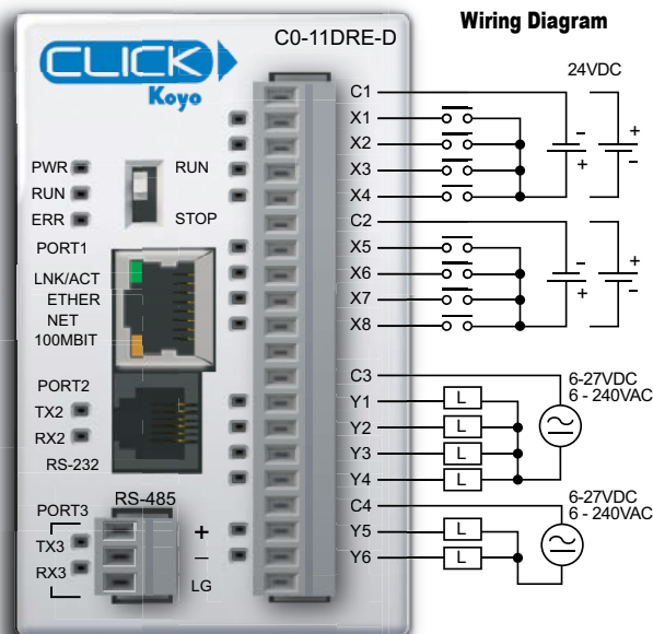
Wiring Diagram
