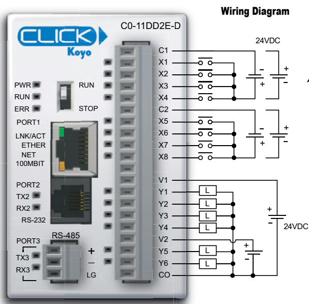
Wiring Diagram
