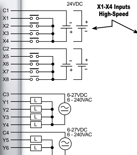
Wiring Diagram
