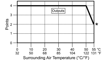
C0-02DR-D Temperature Derating Chart
