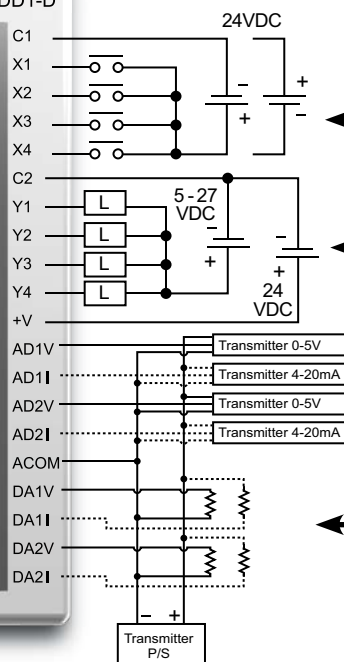
Wiring Diagram
