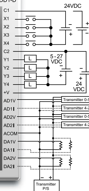
Wiring Diagram
