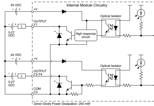
Equivalent Discrete Output Circuit
