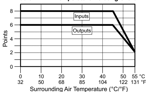
C0-01DD2-D Temperature Derating Chart
