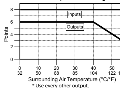
C0-01AR-D Temperature Derating Chart
