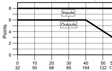
C0-01AR-D Temperature Derating Chart
