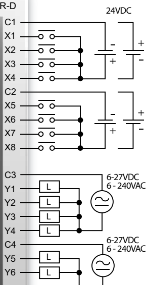
Wiring Diagram
