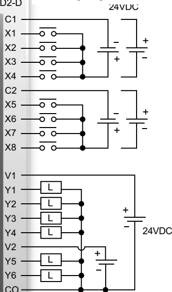
Wiring Diagram
