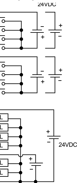
Wiring Diagram
