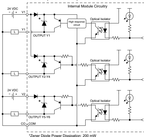
Equivalent Output Circuit
