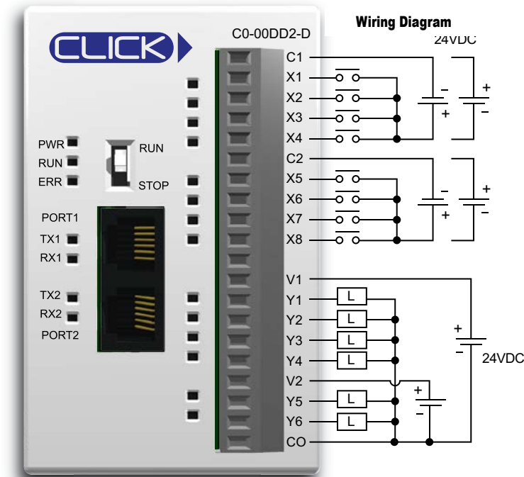
Equivalent Input Circuit
