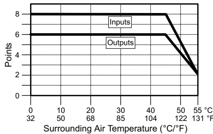
C0-00DD2-D Temperature Derating Chart
