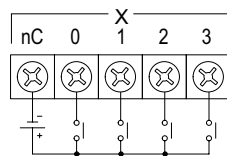
Sinking Input
