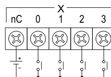
Sourcing Input
