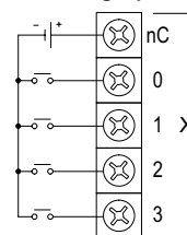
Sourcing Input
