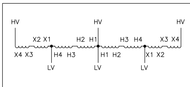
Wiring Diagram 10
