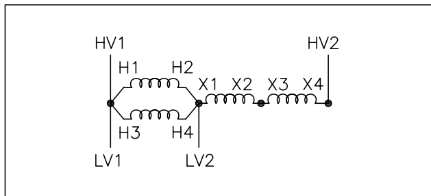
Wiring Diagram 2
