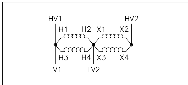
Wiring Diagram 1
