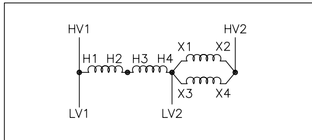
Wiring Diagram 3
