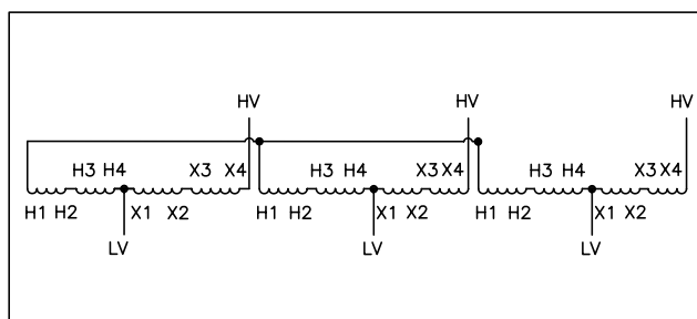
Wiring Diagram 8
