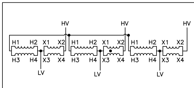
Wiring Diagram 5
