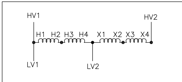
Wiring Diagram 4
