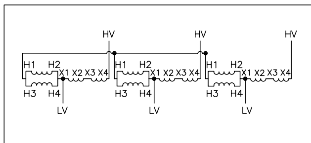
Wiring Diagram 6
