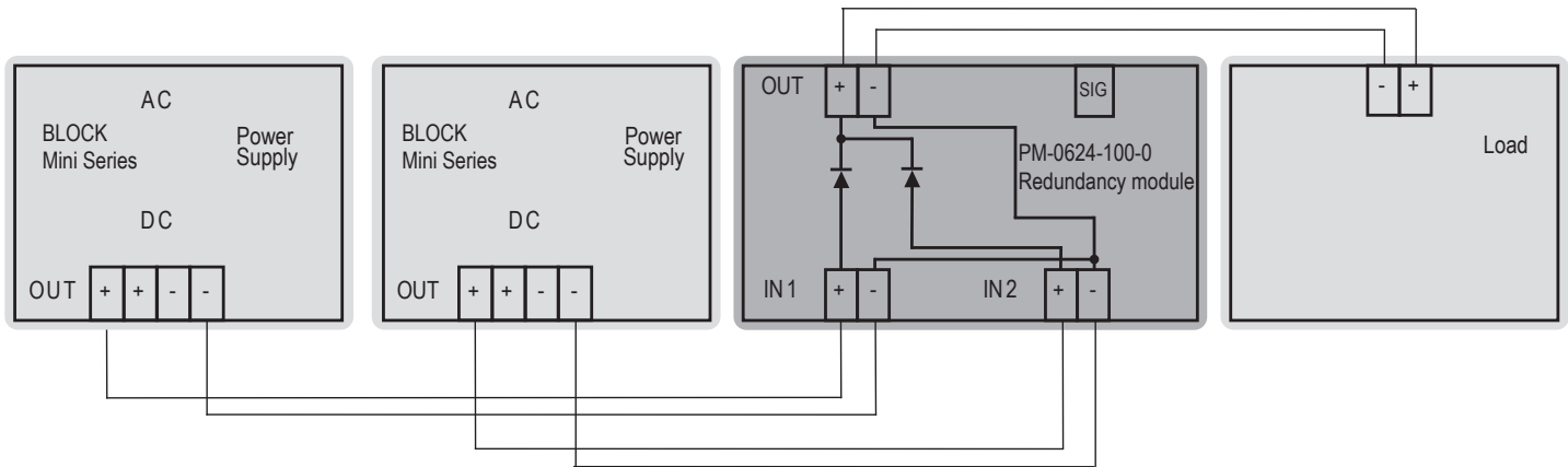
Redundancy Module Function Diagram
