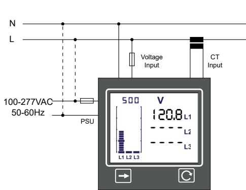
Single phase 2-wire (1P2W)
