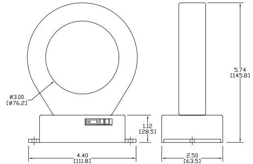
ACTR Series, 750 & 2000 Amp Fixed Core Large Aperture
