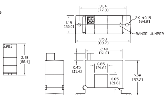
ACTR Series, Up to 200 Amp Split Core
