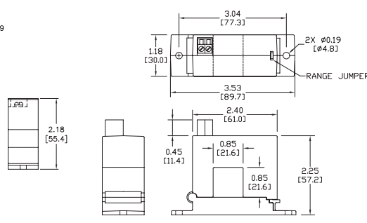
ACTR Series, Up to 200 Amp Split Core
