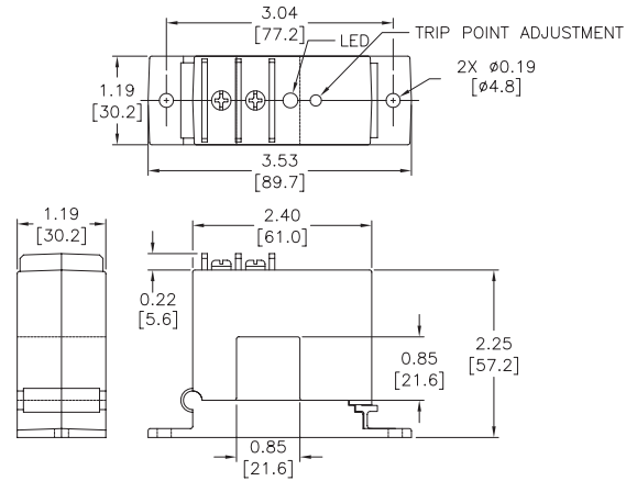
ACS200 Series Split Core
