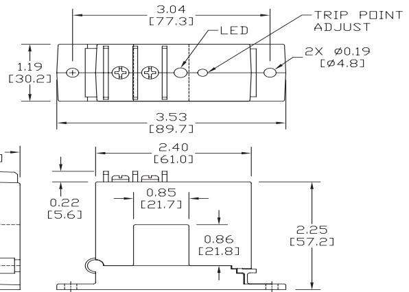
ACS150 Series Split Core
