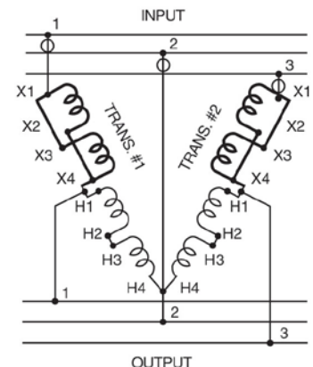
FIG. CC OPEN DELTA
