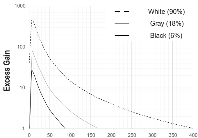
Excess Gain
