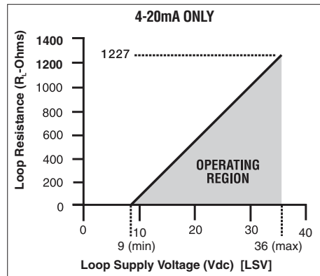
Power Supply Voltage vs Loop Resistance
