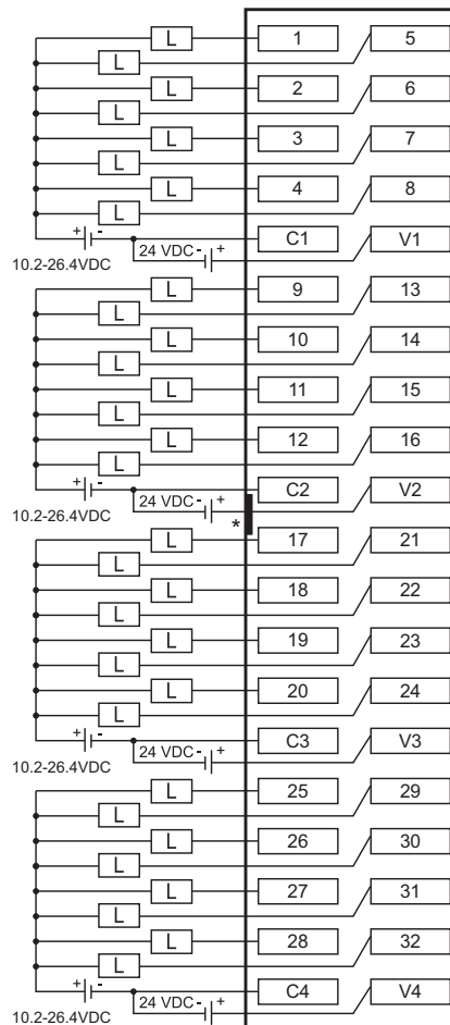
Dual Power Source
