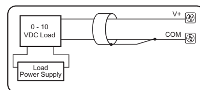
Voltage Output Circuit
