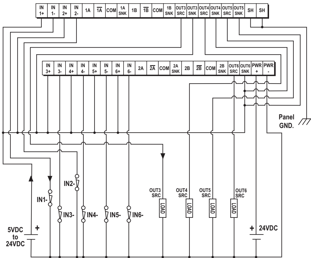
Sourcing I/O Wiring Diagram
