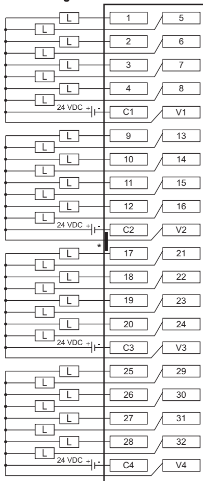
Single Power Source
