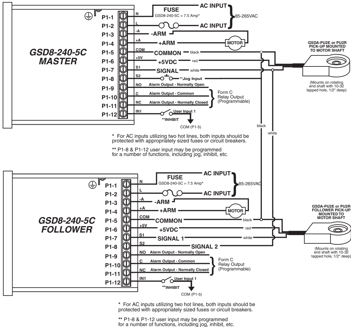
GSD8-240-5C Wiring Diagram
