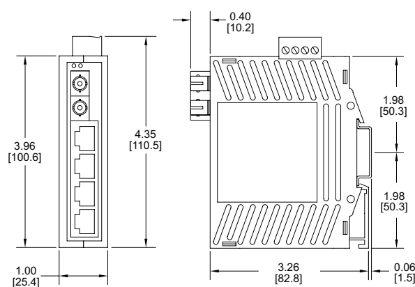
SE-SW5U-SC SE-SW5U-ST
