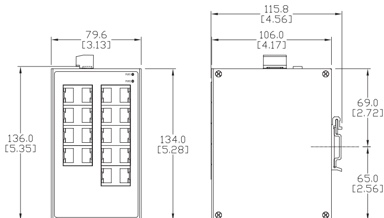
SE2-SW18U-2G-T
