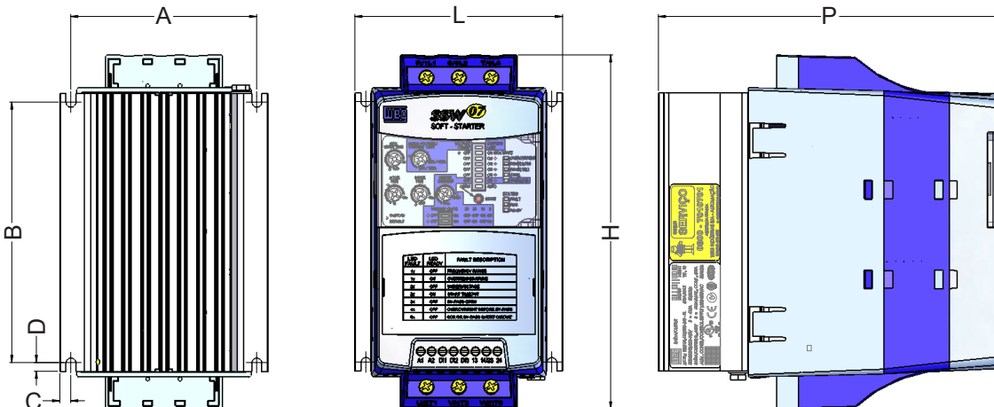
Figure 3.1 - SSW-07 dimensions
