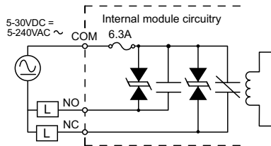
Outputs NO5 / NC5 – NO8 / NC8
