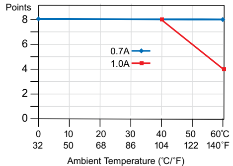
Derating Chart
