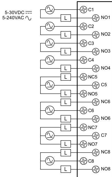
Outputs NO5 / NC5 – NO8 / NC8
