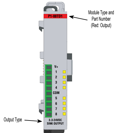
Discrete Output Modules
