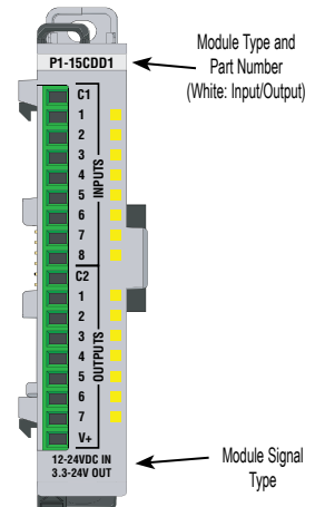
Discrete Input/Output Modules
