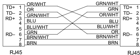
Crossover Cable
