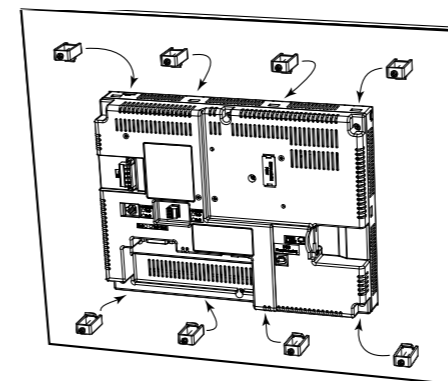
EA9-T10CL (8 places)
