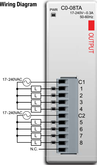
Wiring Diagram
