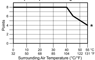
Output Temperature Derating Chart
