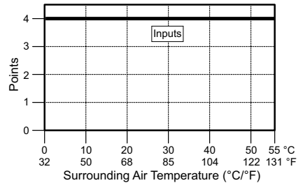
C2-08DR-6C Temperature Derating Chart
