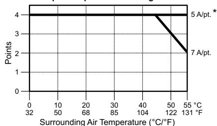
Output Temperature Derating Chart
