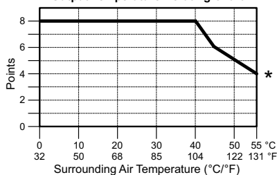
Output Temperature Derating Chart
