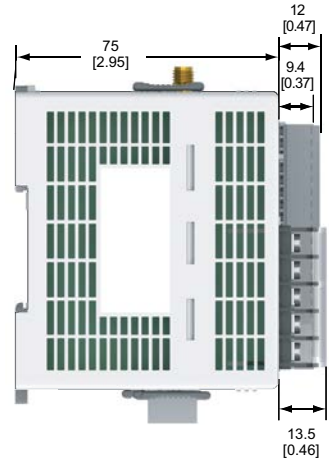
Unit Dimensions mm [inches]
