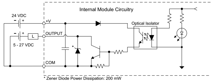
Equivalent Output Circuit
