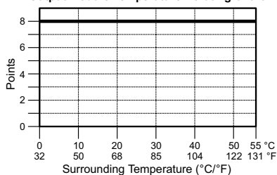
Output Module Temperature Derating Chart
