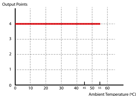
Output Temperature Derating Chart
