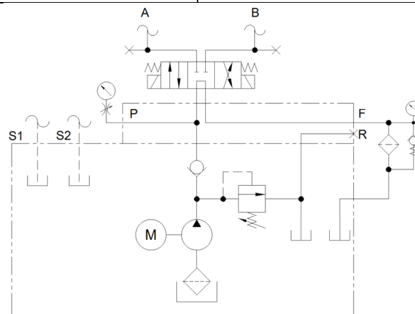
Figure 6 – M4505251-03HM01, M4505351D03HM01 Hydraulic schematic
