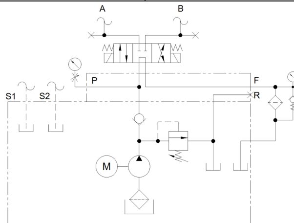
Figure 9 – M4505301-04HN01,M4505351D04HN01Hydraulic schematic
