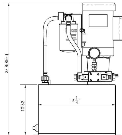
Figure 11 – M4505351D21HR01 Dimensions
