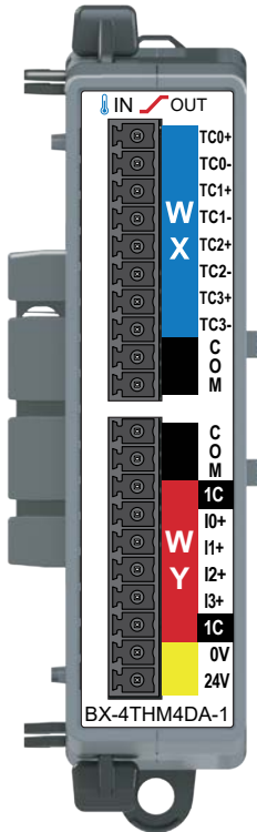
BX-4THM4DA-1 Thermocouple Temperature Input/ Analog Output Expansion Module 4-pt Thermocouple Temperature Input 4-pt Universal Analog Output
