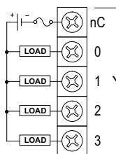
Sinking Output
