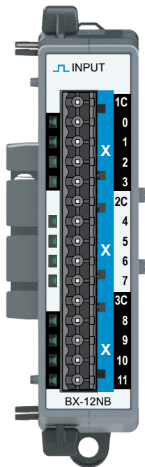
BX-12NB Input Module 12-pt, 12–24 VAC
