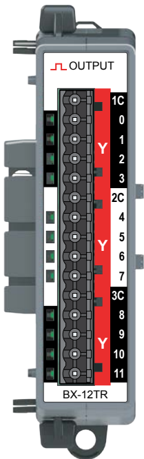
BX-12TR Output Module 12-pt, Relay Form A (SPST)
