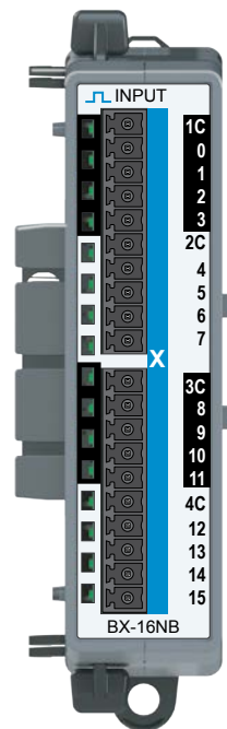
BX-16NB Input Module 16-pt, 12–24 VAC
