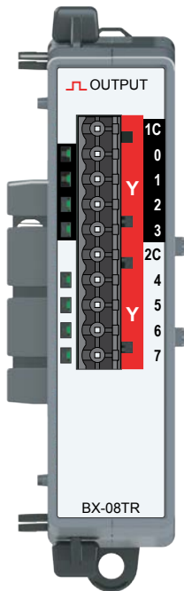
BX-08TR Output Module 8-pt, Relay Form A (SPST)
