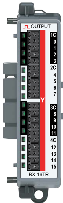
BX-16TR Output Module 16-pt, Relay Form A (SPST)
