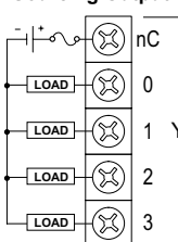
Sourcing Output
