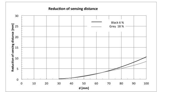
FKLS-*_*-3* (right angle optical head, laser class 1)
