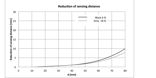
FKLW-*_*-1* (axial optical head, laser class 2)
