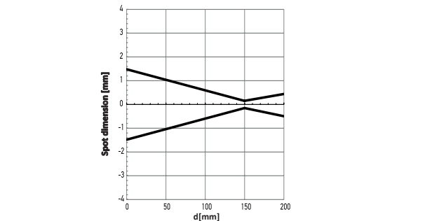
FKLS-*_*-1* (axial optical head, laser class 1)
