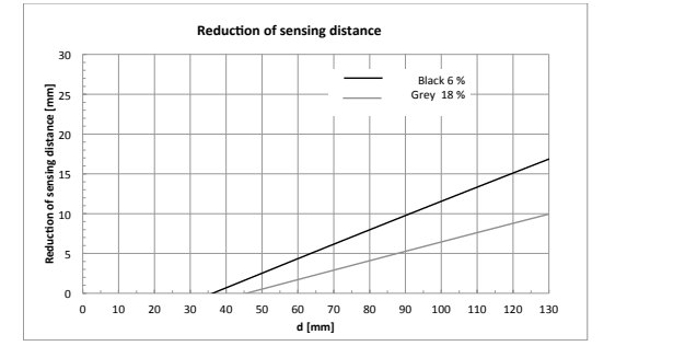
FKLW-*_*-3* (right angle optical head, laser class 2)
