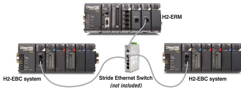
Example of an Ethernet remote I/O system using an H2-ERKIT-2. CPU, bases, I/O modules, Ethernet switch, etc. are sold separately.
