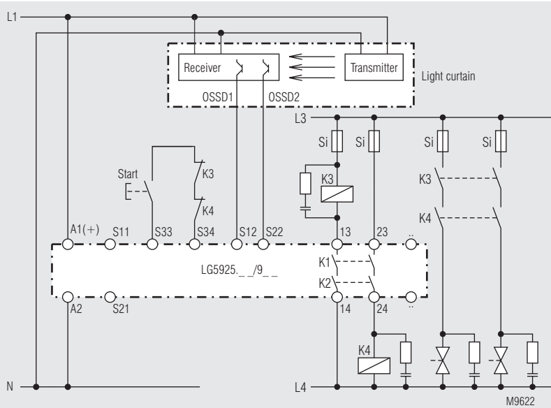
Contact reinforcement and contact extension by external contactors
