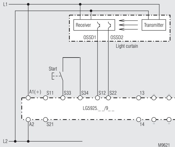
Two channel connection of light curtains with selftest according to EN 61496-1.
